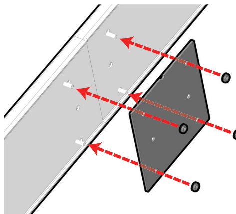
Inside Joiner Plate
